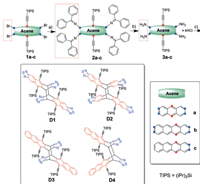
Scheme 1. Synthetic route for D1–4 : a) benzophenone imine, rac -BINAP, Pd 2 (dba) 3 , t BuONa, toluene, 110 °C, 55–65 %; b) 2.0 M HCl, THF, r.t. 90–95 %; c) TMS-Cl, PhNSO, Py, 80 °C, 57–77 % ( D1–3 ) and 15 % ( D4 ). Blue and red dots on acenes a , b , and c represent the substitution of corresponding functional groups. BINAP = 2,2'-bis(diphenylphosphino)-1,1'-binaphthyl, dba = dibenzylideneacetone, TMS-Cl = trimethylsilyl chloride, PhNSO = thionylaniline, and Py = pyridine.
